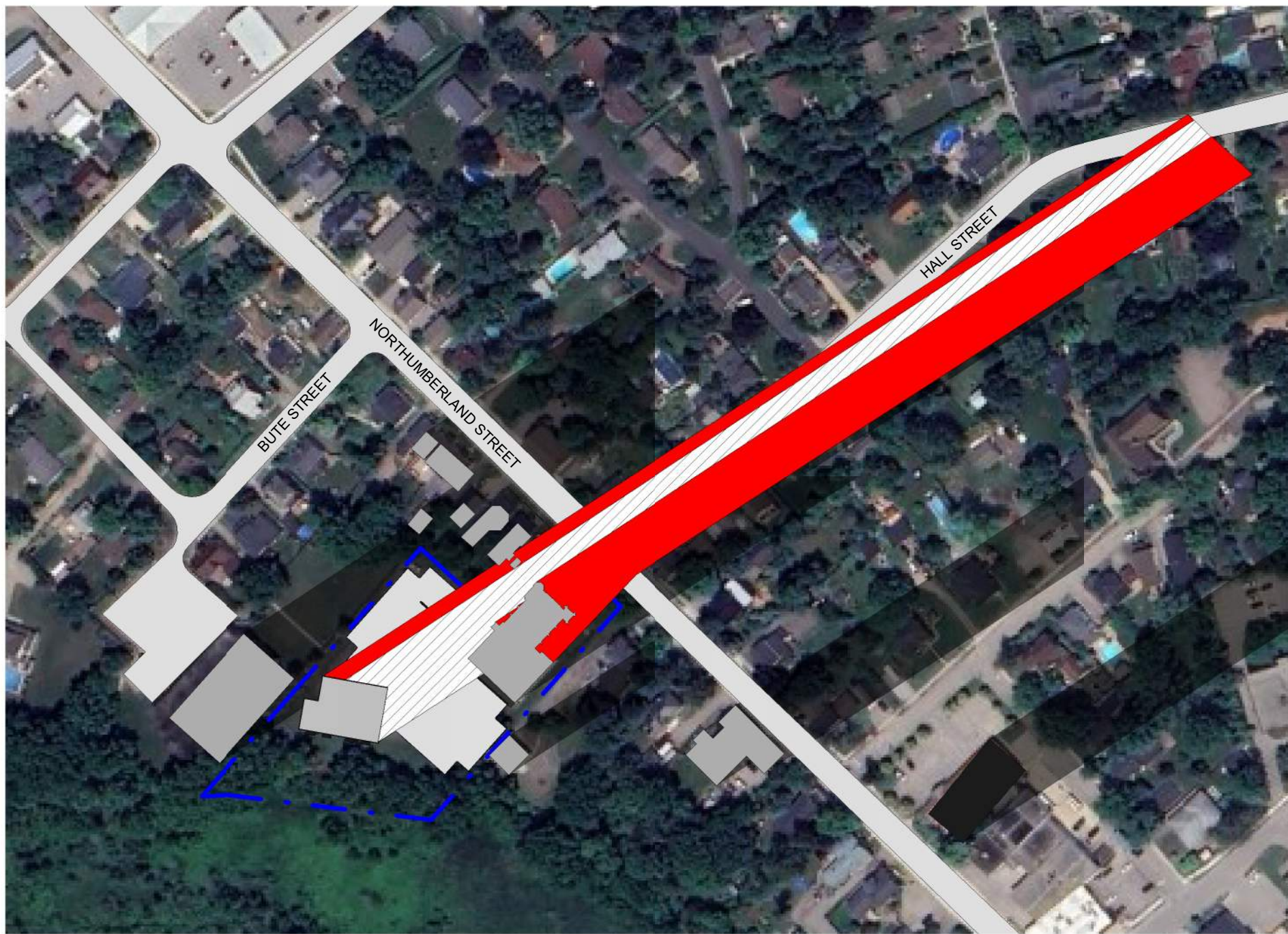
9 Shadow Study December 21 5pm 1 : 2000
