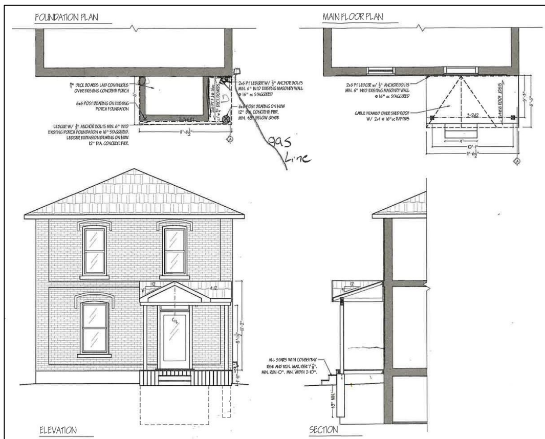
Figure 2: Proposed Elevation
