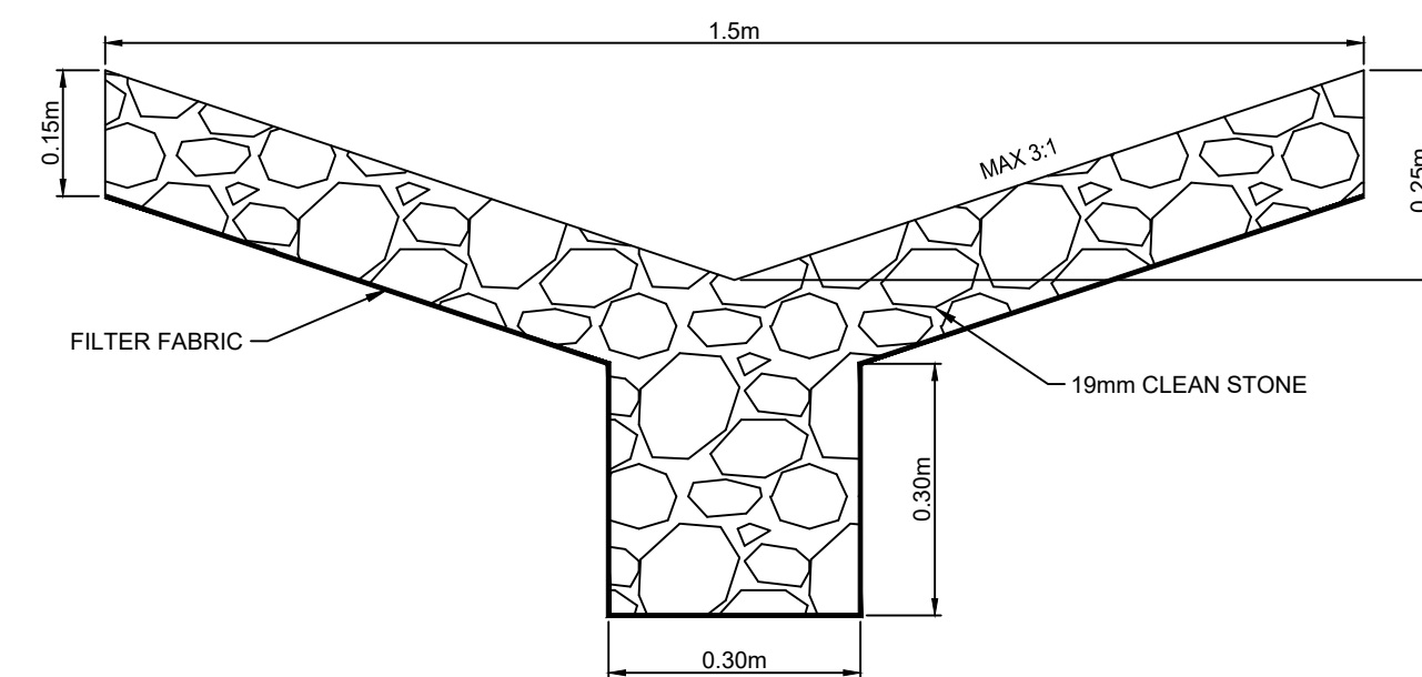
TYPICAL DITCH DETAIL NOT TO SCALE
